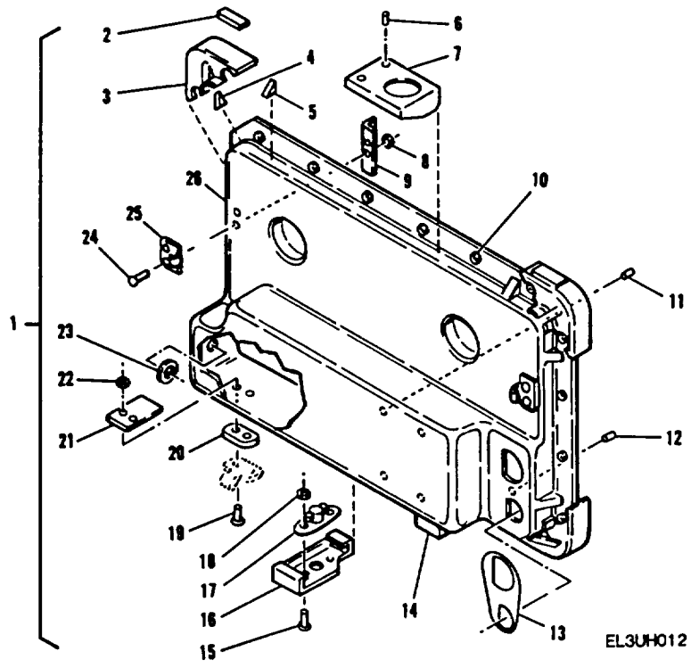
Figure 11. Antenna Housing.
