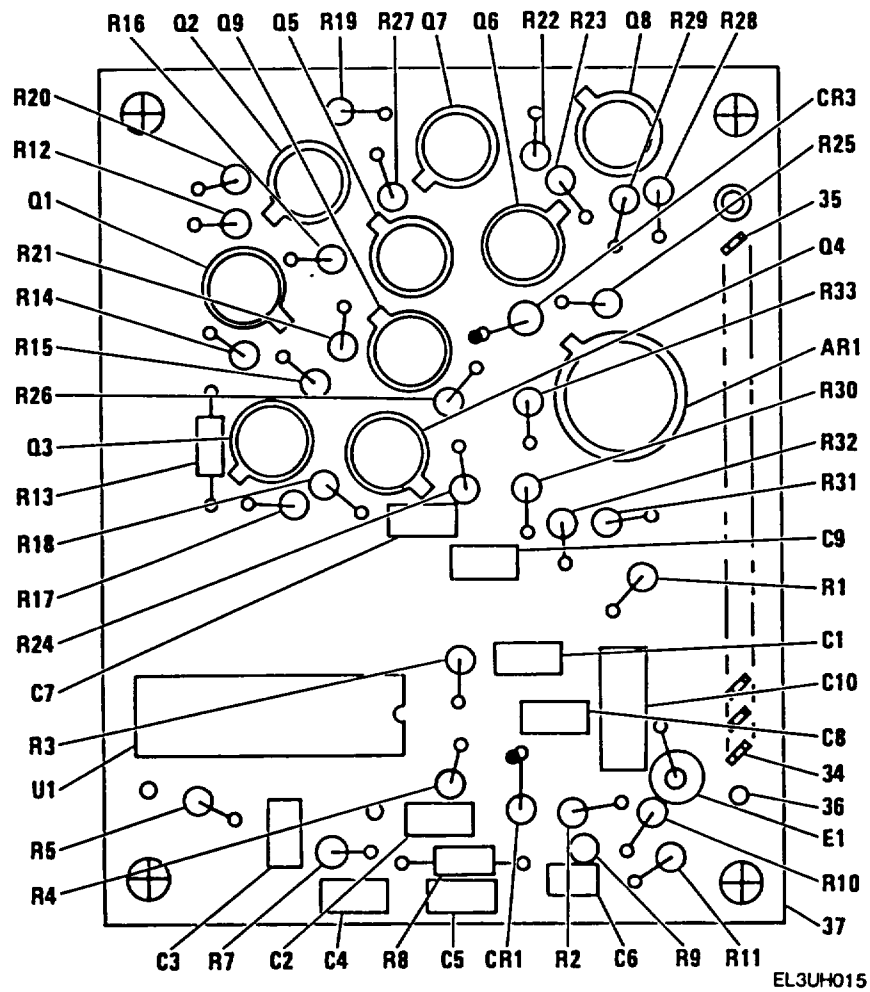
Figure 13. Antenna Circuits Circuit Card.
