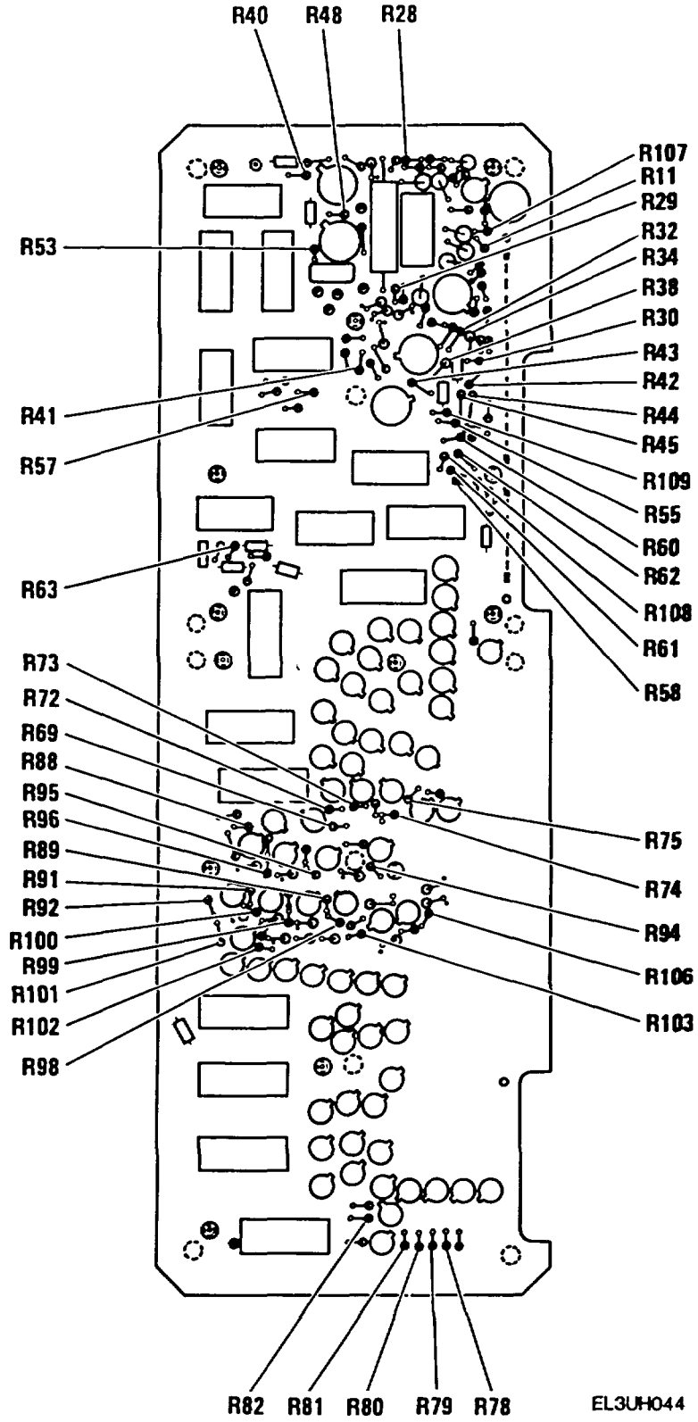
Figure24. Digital Processor Circuit Card (Sheet 5 of 6)
