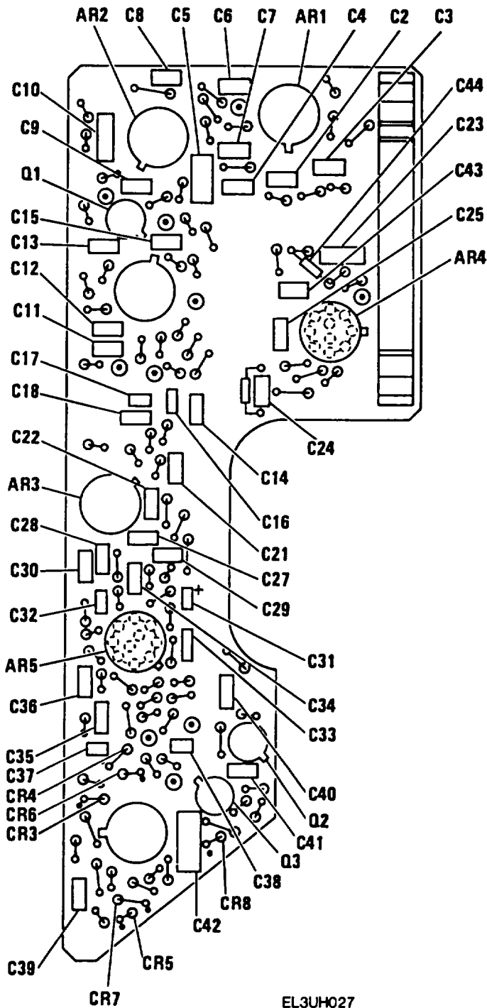
Figure 19. All Range Circuit Card (Sheet 1 of 3).
