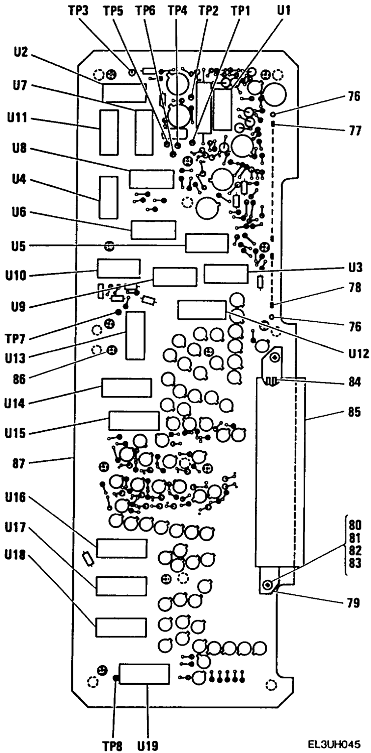
Figure24. Digital Processor Circuit Card (Sheet 6 of 6).
