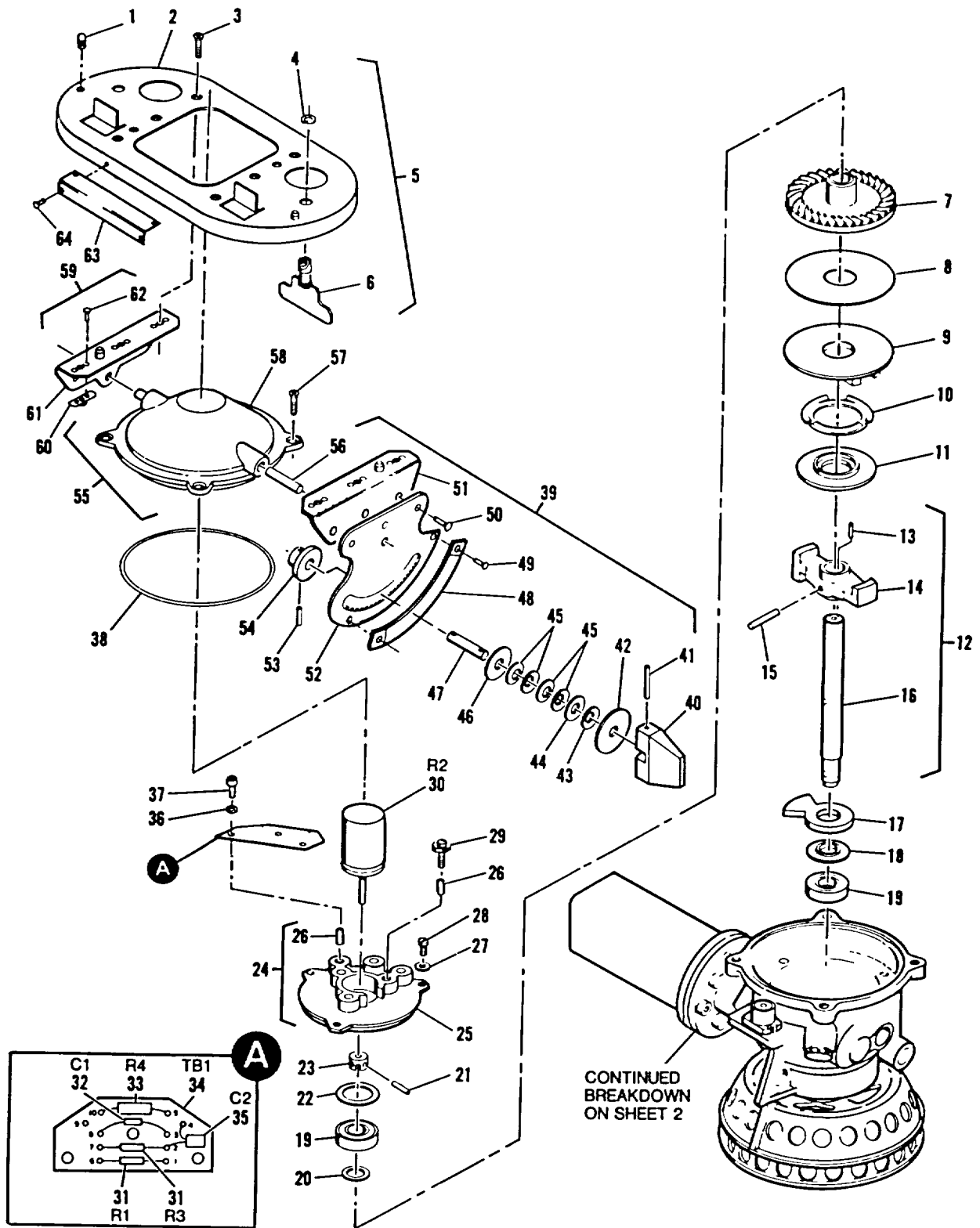
Figure 2. Antenna Drive AB-1205A/PPS-15(V) (Sheet 1 of 2)
