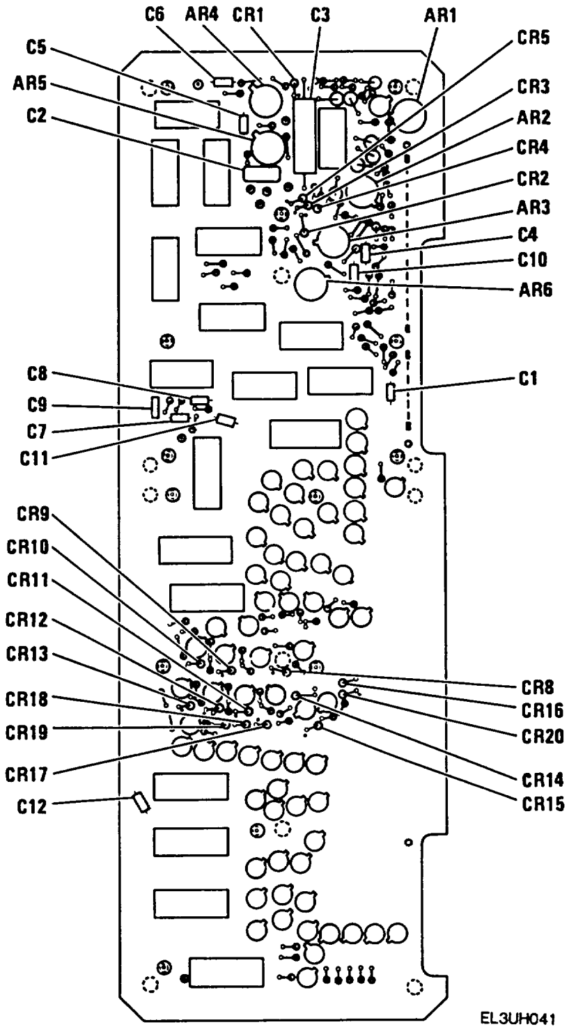
Figure 24. Digital Processor Circuit Card (Sheet 2 of 6).
