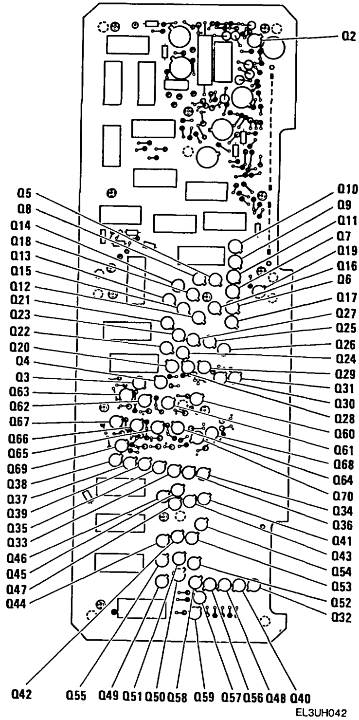
Figure 24. Digital Processor Circuit Card (Sheet 3 of 6).
