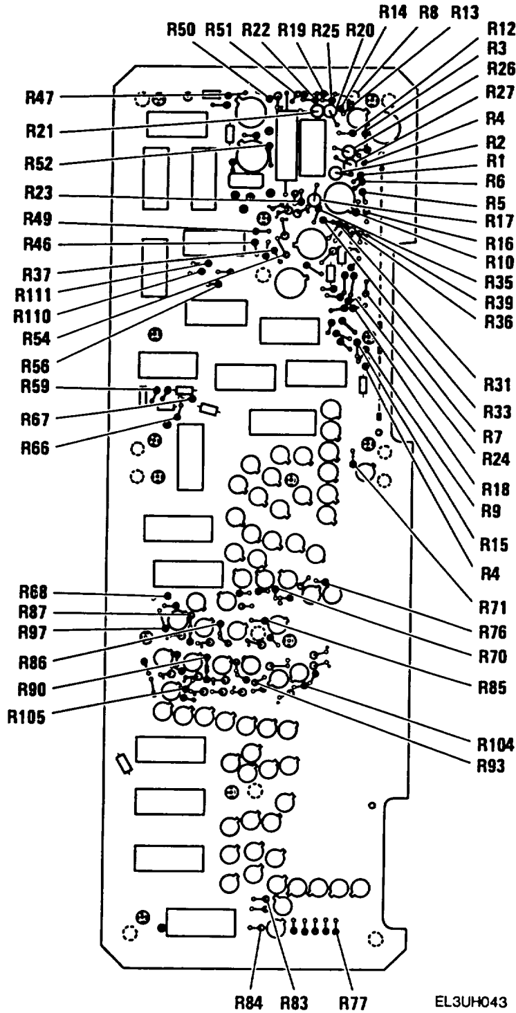
Figure 24. Digital Processor Circuit Card (Sheet 4 of 6).
