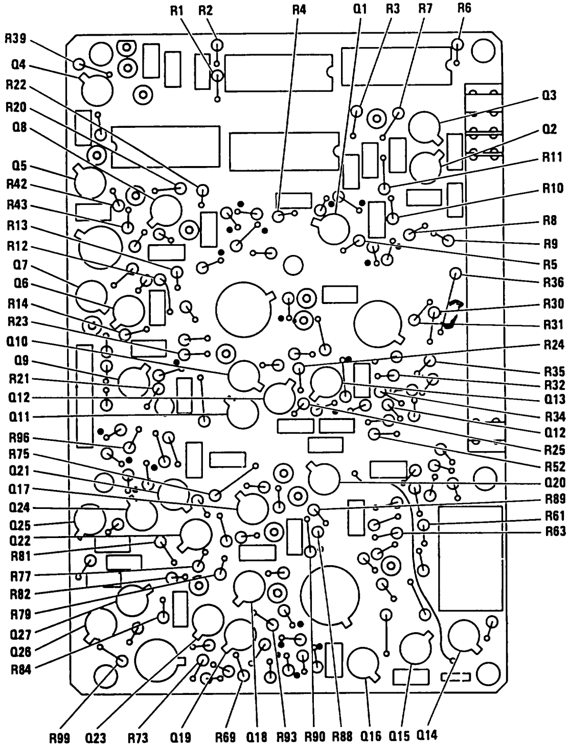
Figure 21. Discrete Range Circuit Card (Sheet 3 of 5).
