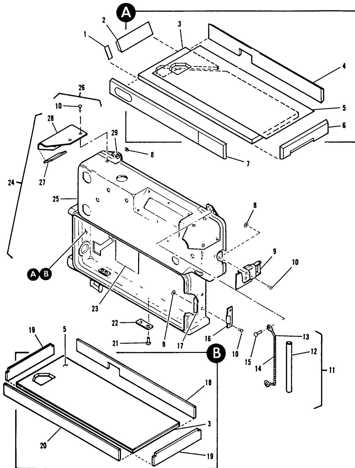
Figure 15. Housing.
