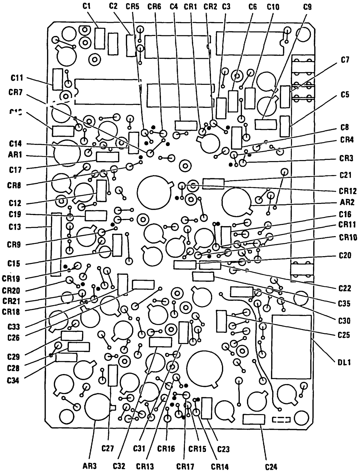
Figure 21. Discrete Range Circuit Card (Sheet 2 of 5)
