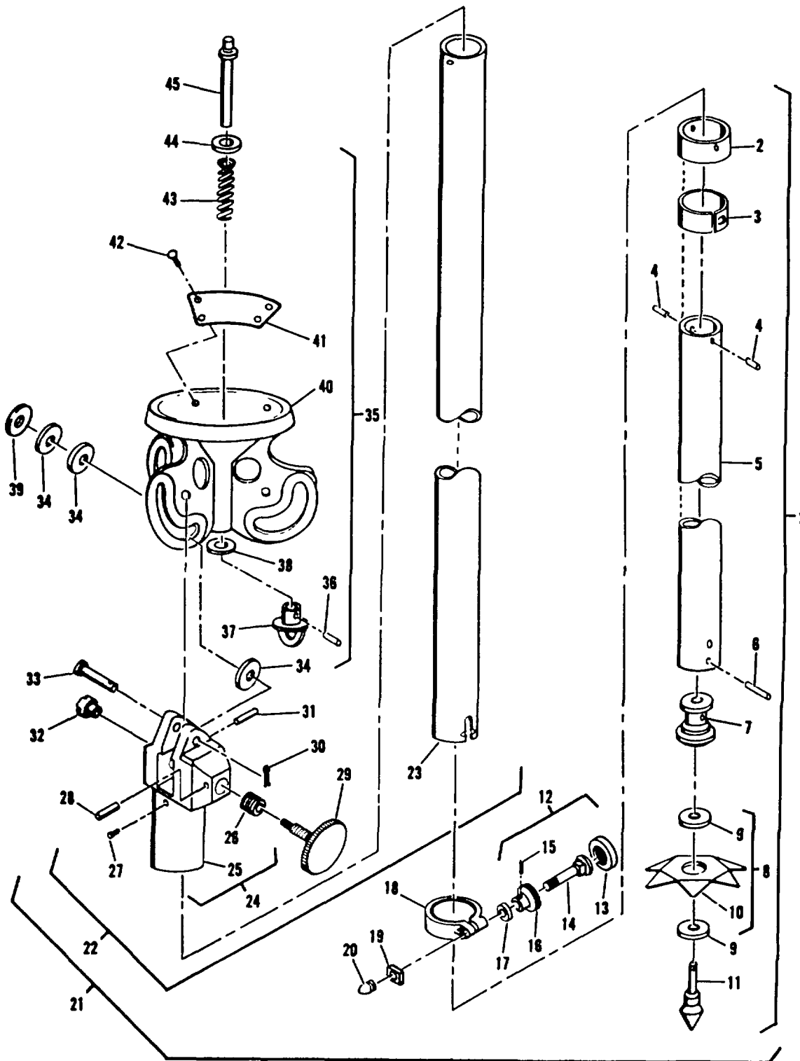
Figure 3. Radar Tripod MT-4800/PPS-15(V).
