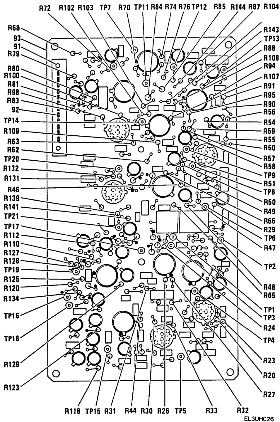
Figure 18. Automatic Alarm Circuit Card (Sheet 6 of 6).
