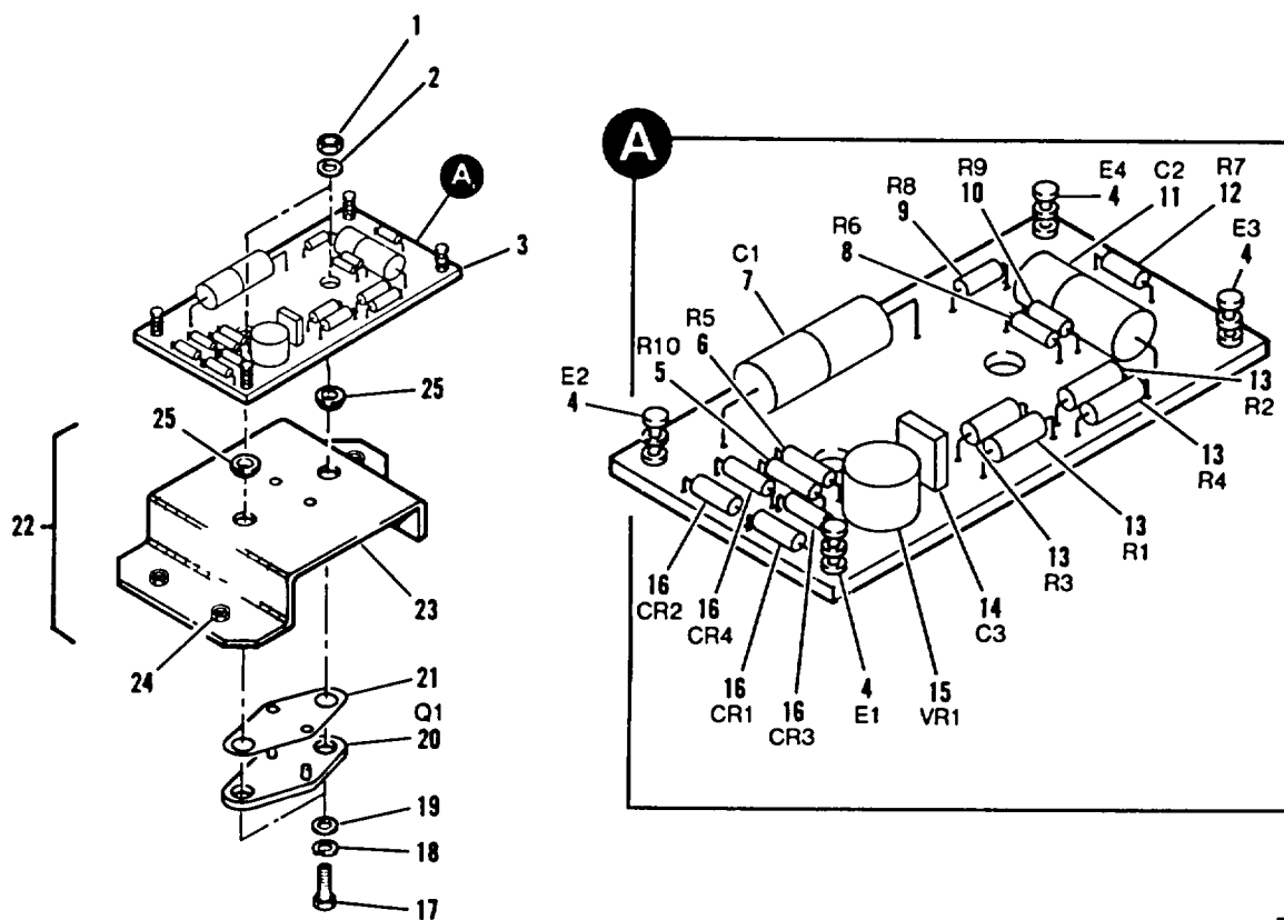
Figure 6. Power Regulator Circuit Card
