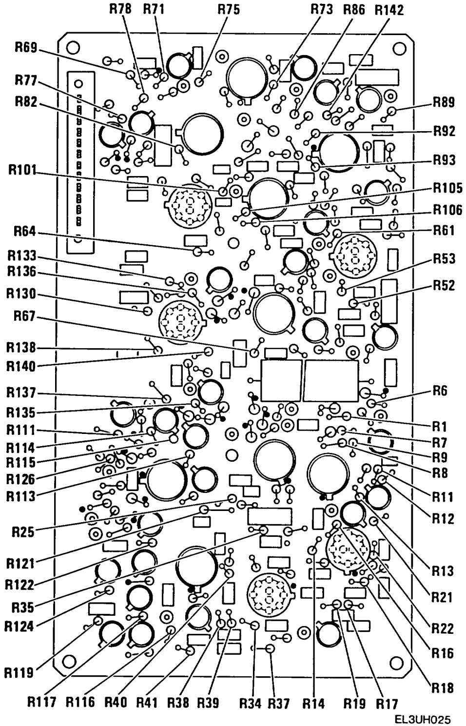
Figure 18. Automatic Alarm Circuit Card(Sheet 5 of 6)
