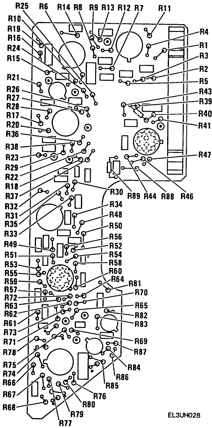
Figure 19. All Range Circuit Card (Sheet 2 of 3)
